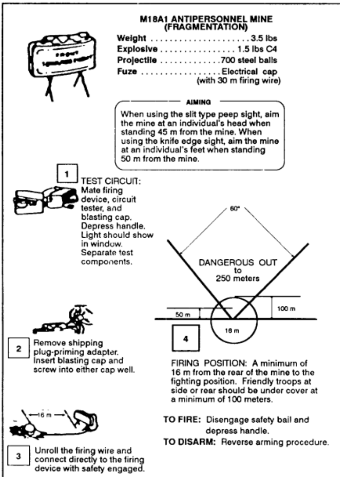
Figure B-8. Antipersonnel mines (continued).
