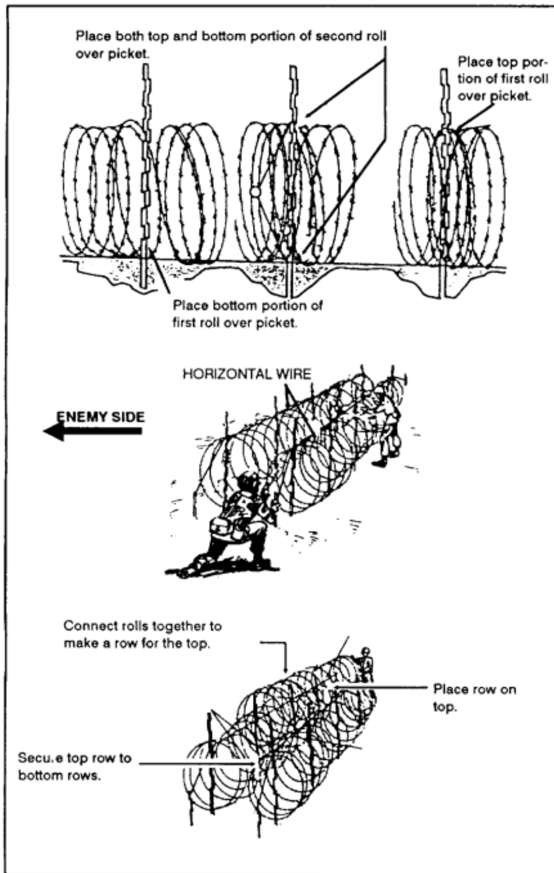
Figure 2-76. Concertina fence (continued).
