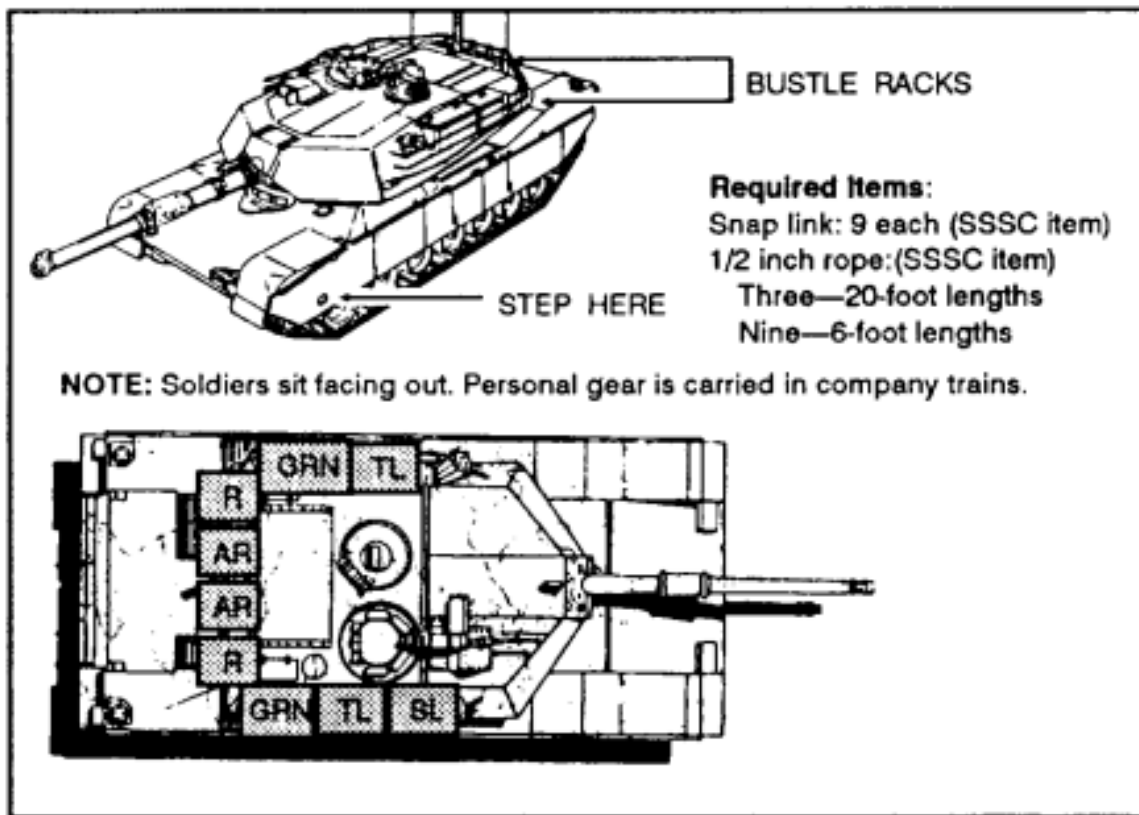
Figure 2-74. Mounting and riding arrangements on an M1.
