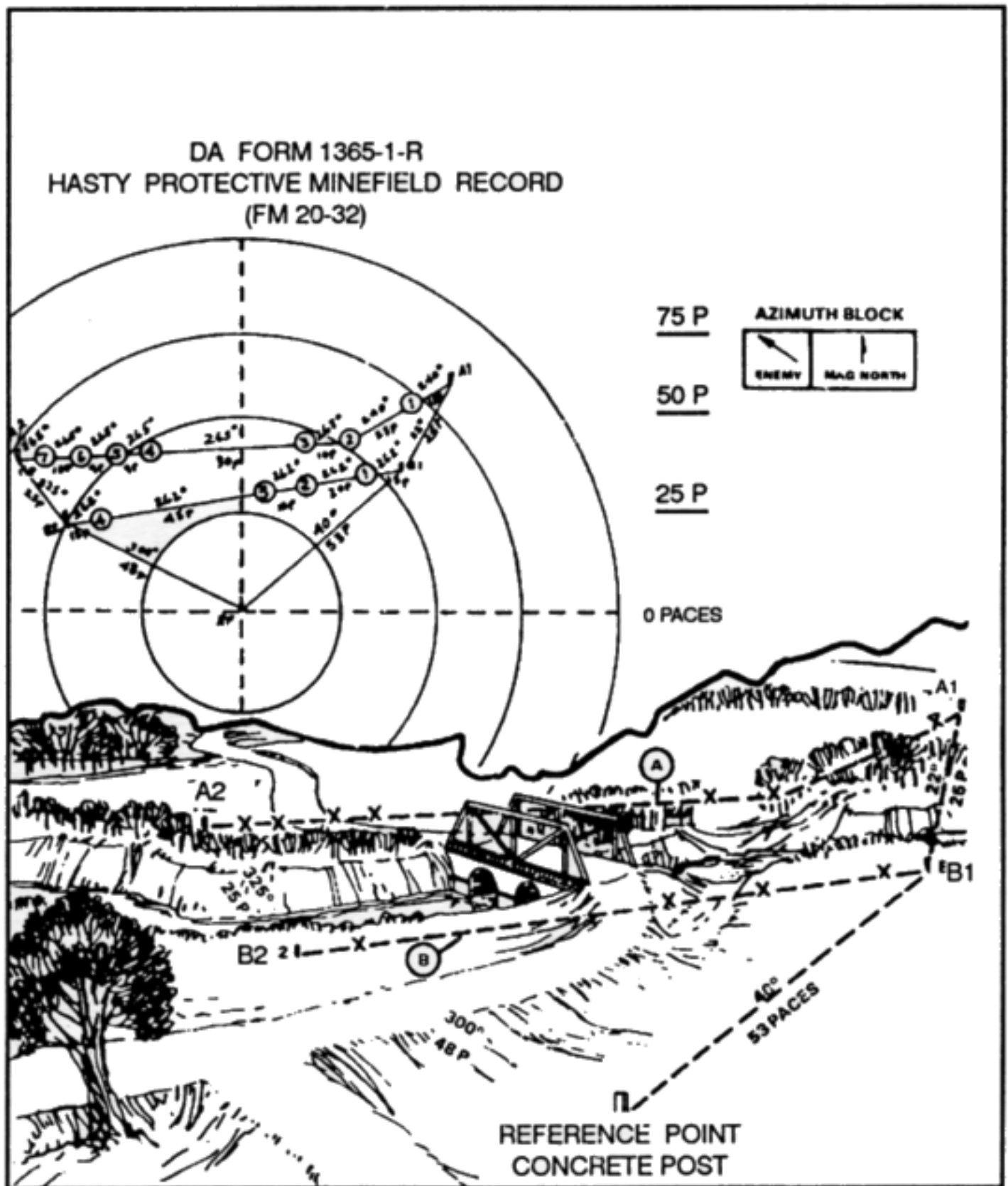
Figure 2-80. Marking and recording minefield (continued).
