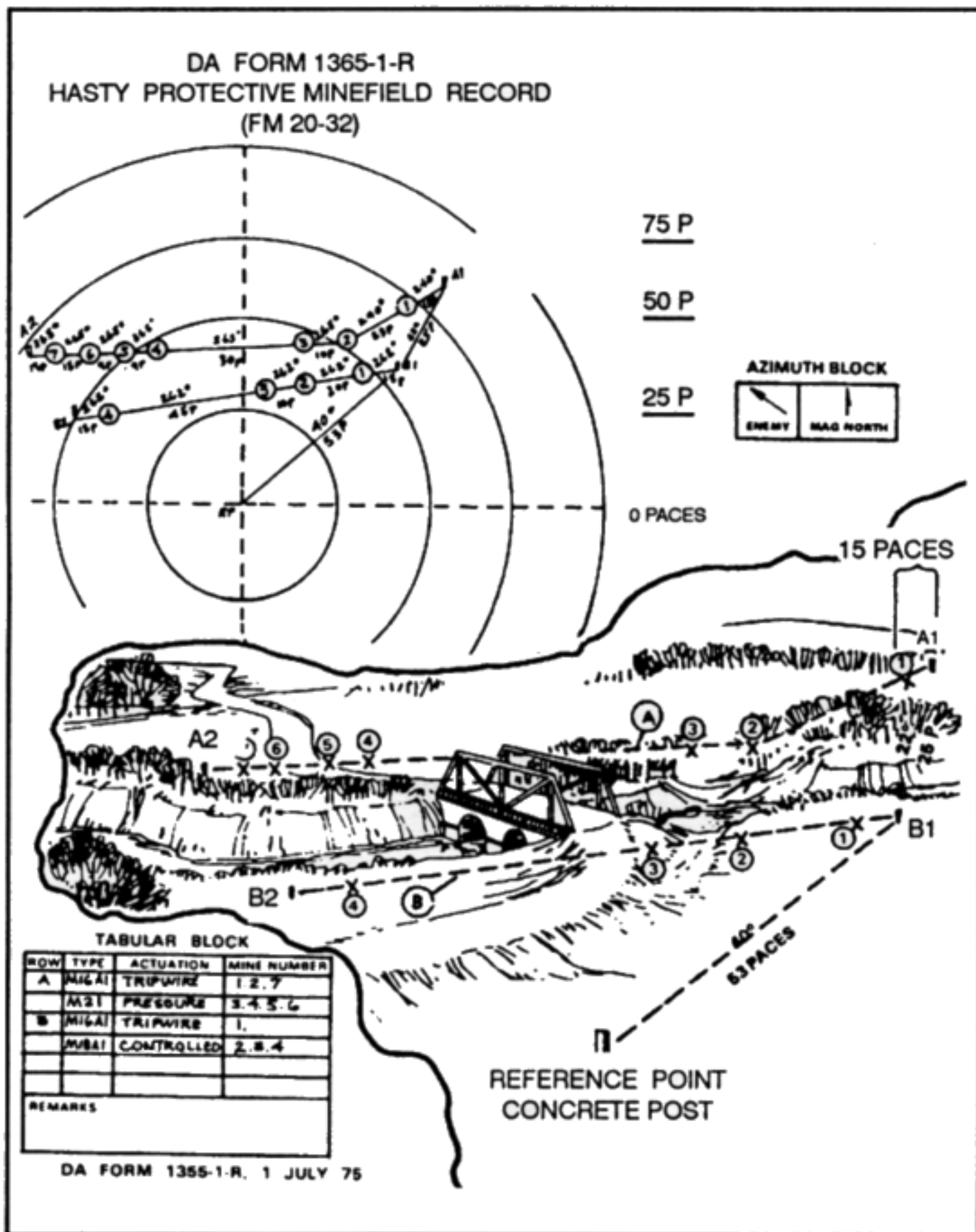
Figure 2-80. Marking and recording minefield (continued).
