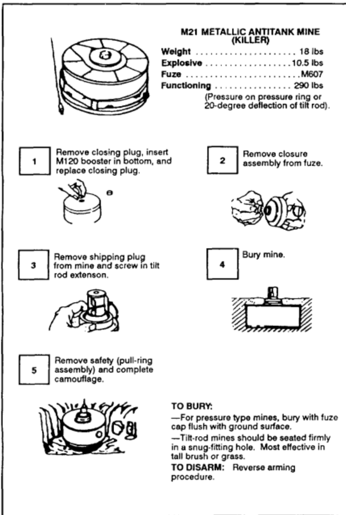
Figure B-9. Antitank mines (continued).
