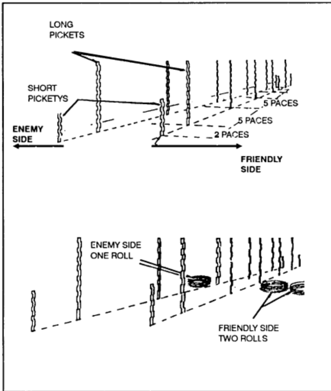
Figure 2-76. Concertina fence.
