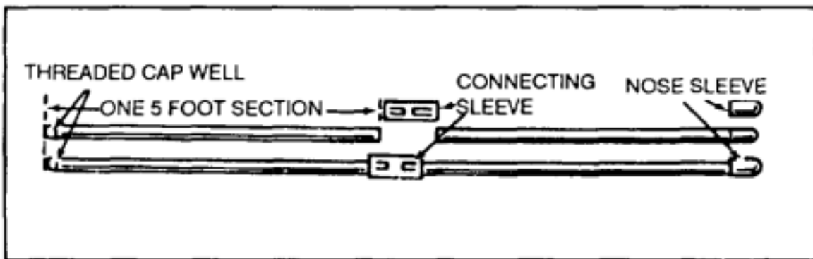
Figure 2-81. Bangalore torpedo.
