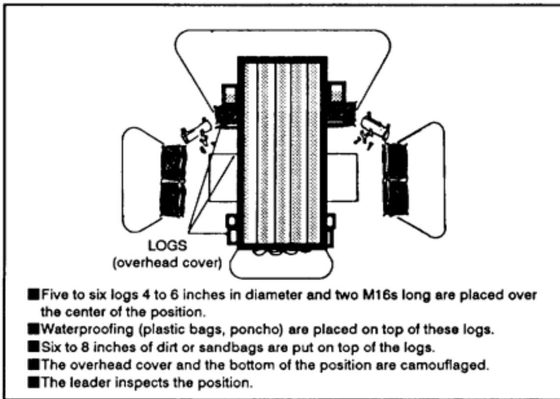
Figure 2-47. Stage 4, preparation of a fighting position.
